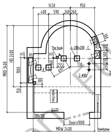
Machine room plan/1:60
