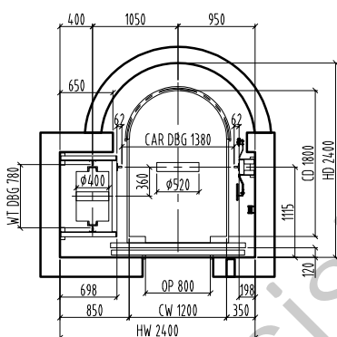
Hoistway plan/1:60
