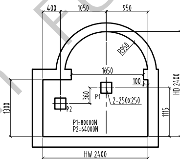
Pit plan/1: 60
